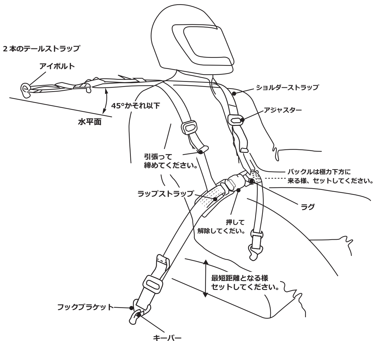
Fig 1- 全体構成図 -Supersports (FOR 2SEATER SPORTS VEHICLE)
